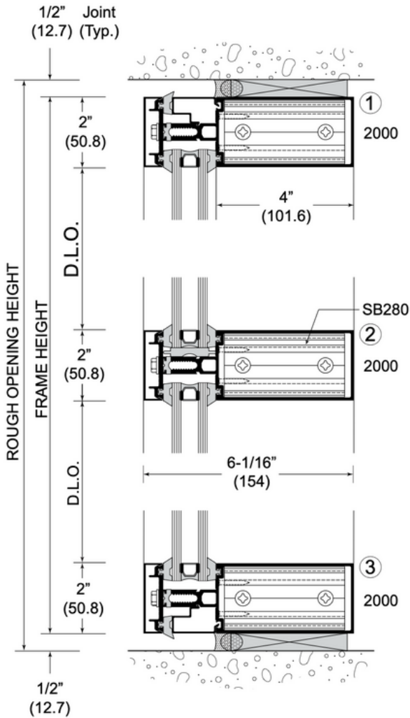
TYPICAL ELEVATION
