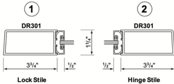
OFFSET HUNG DOORS
