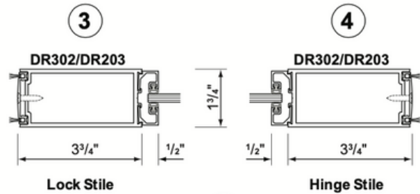
CENTER HUNG DOORS
